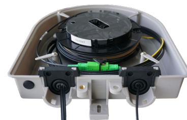
6" Flange Deploy Reel (Installed)
